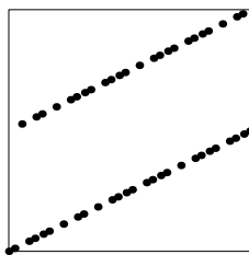
Figure 3.5: The unit square with (n\theta_1, n\theta_2) \bmod 1 for \theta_1 = 2\sqrt{2} , \theta_1 - 2\theta_2 = 2 and n = 0, \dots, 50 .
