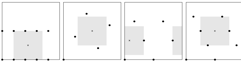
Figure 3.2: The unit square with the set \{n(\frac{u_1}{v_1}, \frac{u_2}{v_2}) \bmod 1 : n \in \mathbb{N}\} for (\frac{u_1}{v_1}, \frac{u_2}{v_2}) = (\frac{1}{5}, \frac{1}{2}), (\frac{1}{5}, \frac{2}{5}), (\frac{1}{6}, \frac{2}{3}) and (\frac{3}{8}, \frac{1}{4}) , respectively.
