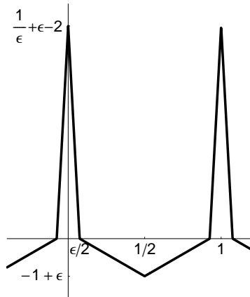
Figure 3.6: The function H
