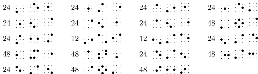
FIGURE 4. The 19 non-Hadamard 3D models with a zero orbit sum, with the order of the associated group. The first one on the second line is the natural 3D analogue of Kreweras’ model.
