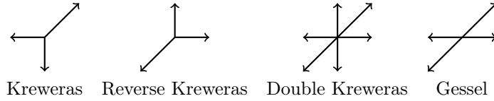
FIGURE 2. The four quadrant models with orbit sum zero: all of them are algebraic.
