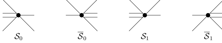
FIGURE 5. Four interesting quadrant models with repeated steps, only differing by a symmetry of the square. All are D-finite, and \bar{S}_1 is even algebraic. See Section 7.2 for S_0 and \bar{S}_0 , Section 8.1 for \bar{S}_1 and Section 8.2 for S_1 . Note that with only one copy of the repeated step, none of these models would be D-finite [8].
