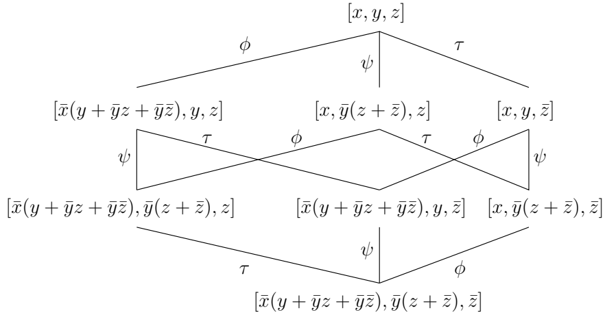
FIGURE 3. The orbit of [x, y, z] under the group generated by \phi , \psi and \tau , when \mathcal{S} = \{\bar{1}\bar{1}\bar{1}, \bar{1}\bar{1}1, \bar{1}10, 100\} .
