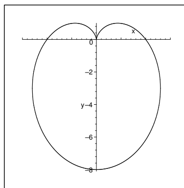
Fig. 4.3.4 cardioid
