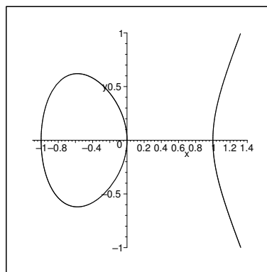
Fig. 4.3.2 elliptic curve
